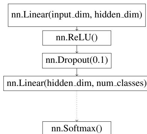
Figure 2: Classifier head used for BERT-based models and FastText for text representation for SA.
