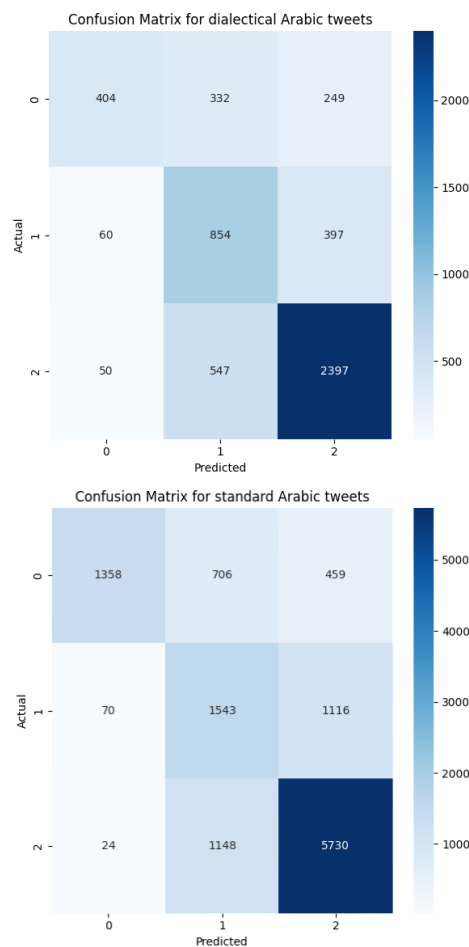
Figure 3: Confusion Matrices for GPT-4-Turbo model evaluation on MAC across different classes (negative, neutral and positive).
