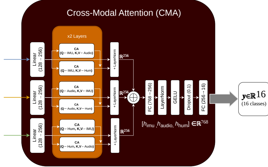
Fig. 11. Cross-Modal Attention (CMA)
