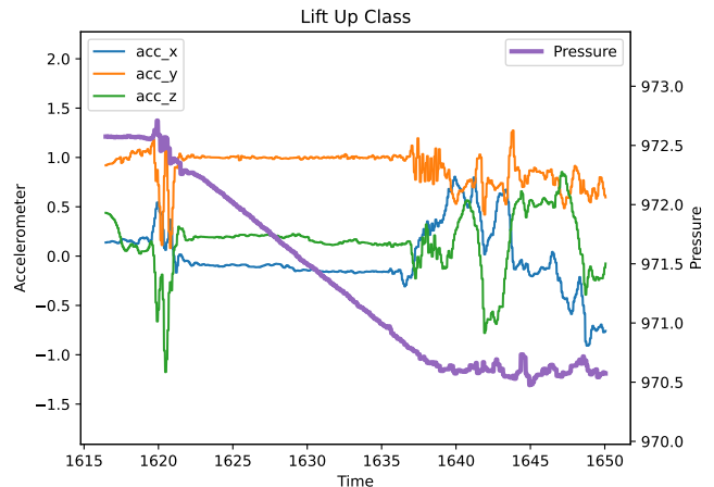
Figure 3: Example accelerometer and barometer data for the 'Lift Up' activity class. While the lift is moving, the participant mostly stood still. We observe the pressure decreasing smoothly.
