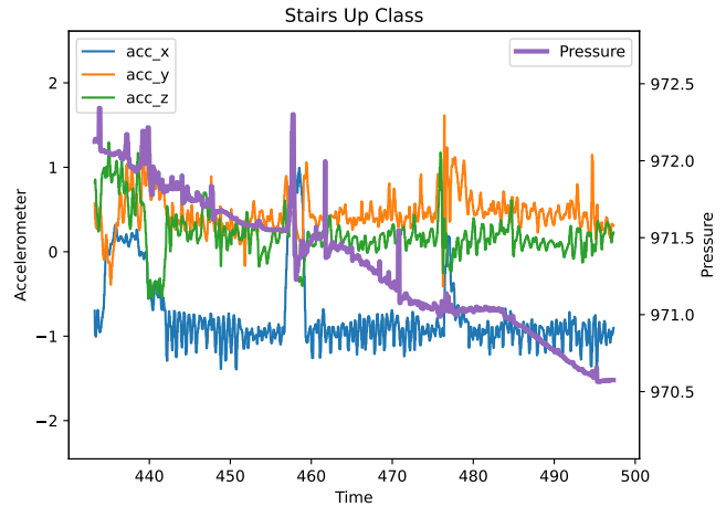
Figure 2: Example accelerometer and barometer data for the 'Stairs Up' activity class. The accelerometer shows the typical patterns of walking. Meanwhile, the pressure steadily decreases, with short plateaus occurring on the stairway's landings. Additionally, the pressure sensor shows some spikes which are likely caused by the movement of the arm while walking.
