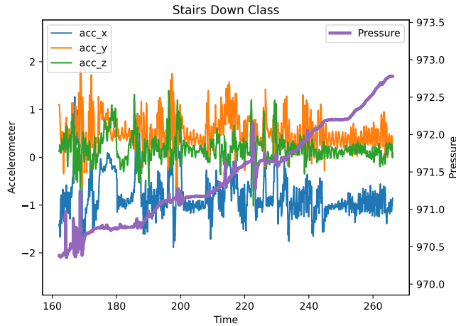
Figure 4: Example accelerometer and barometer data for the 'Stairs Down' activity class. The accelerometer shows a lot of activity, with similar walking patterns as in 'Stairs Up'. In direct comparison, the magnitude and frequency of the movement sensors seem higher. The barometer detects the steadily rising pressure, also interrupted by short plateaus caused by the landings.
