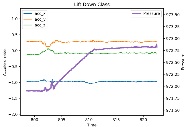
Figure 5: Example accelerometer and barometer data for the 'Lift Down' activity class. The specific participant for this instance was standing very still during the descent. We can see the pressure increasing linearly and smoothly.
